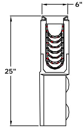
Channel Inlet Options (Ends Only) Plan View N.T.S. NOTE: SEE DRWG 1670 FOR ALTERNATE CONCRETE SURROUND
