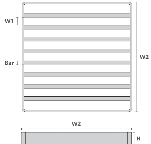
12" HD 304/316L part no. 408045/408145
