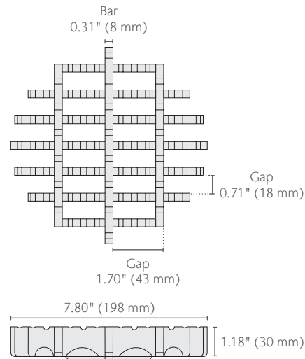
9" Round Frameless Ladder Grate - M125
