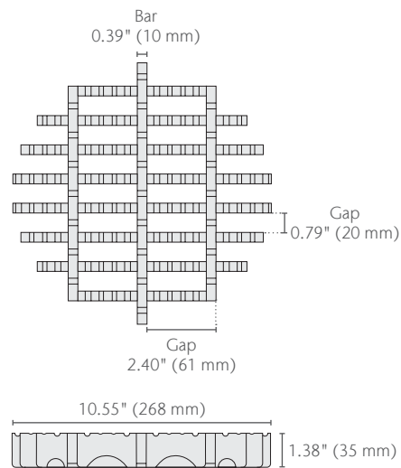
12" Round Frameless Ladder Grate - M 125
