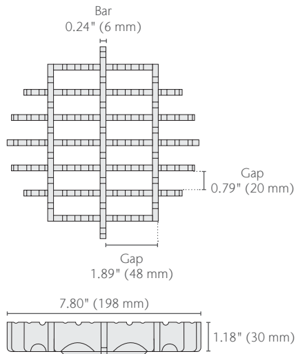
9" Round Frameless Ladder Grate - R50
