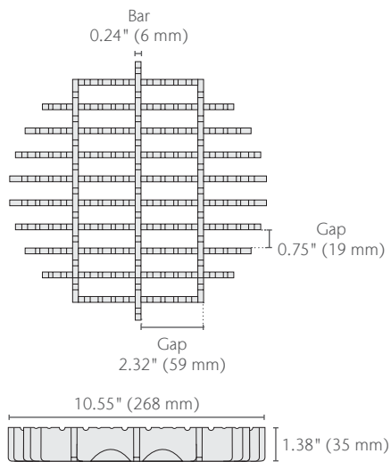
12" Round Frameless Ladder Grate - R50
