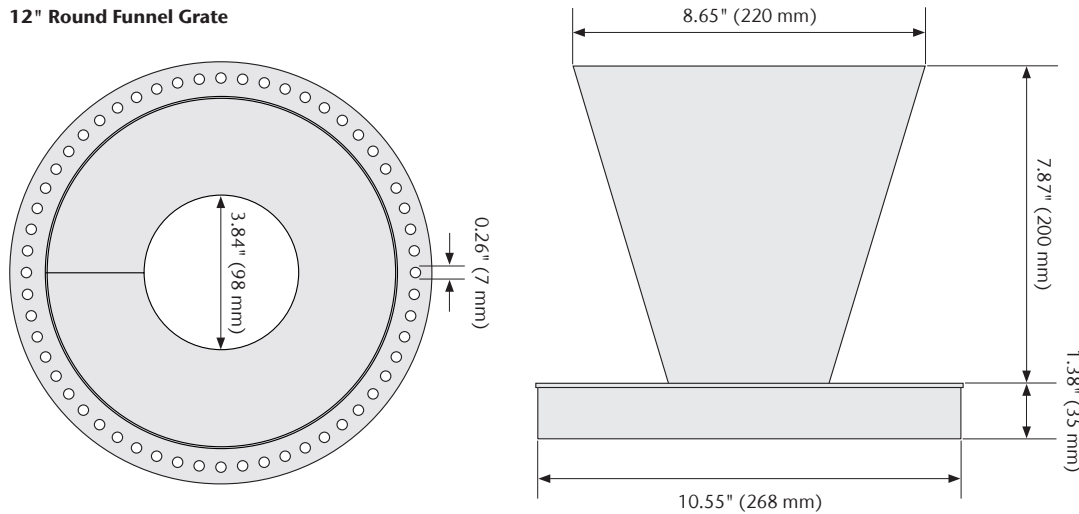
12" Round Funnel Grate
